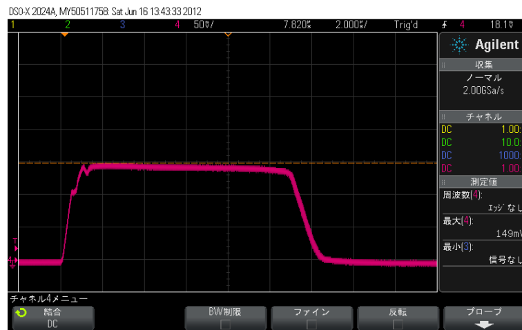
CH4(B)Output Current
