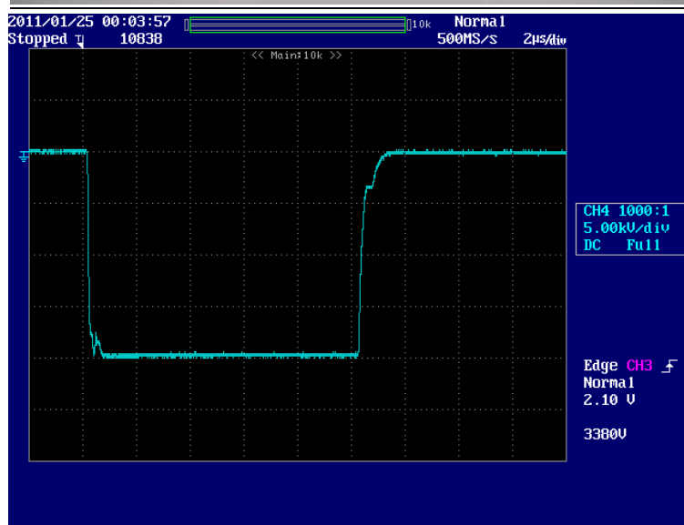
CH4(青):出力電圧 5kV/div 2 \mu s/div
